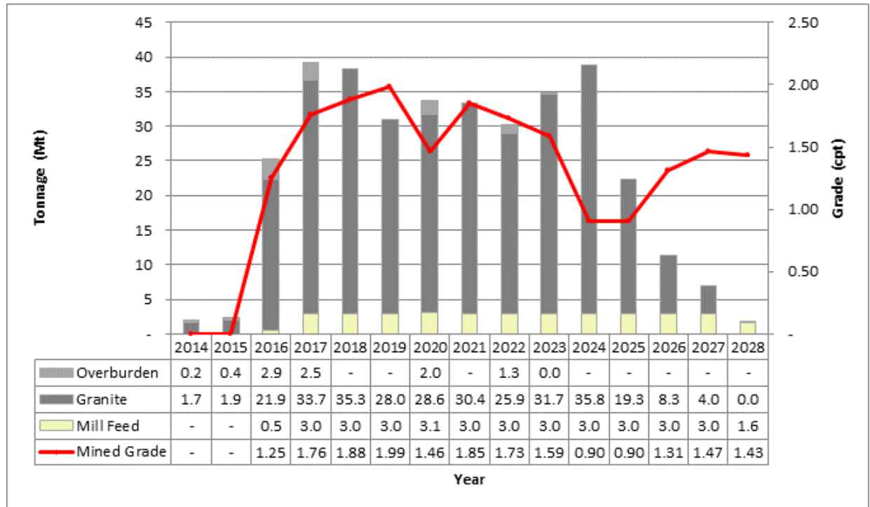
Figure 16-4: Annual Tonnes Mined & Grade
