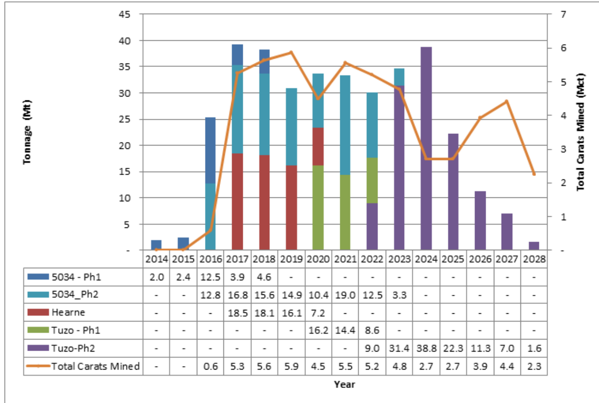
Figure 16-5: Tonnes Mined by Pit & Mined Carats
