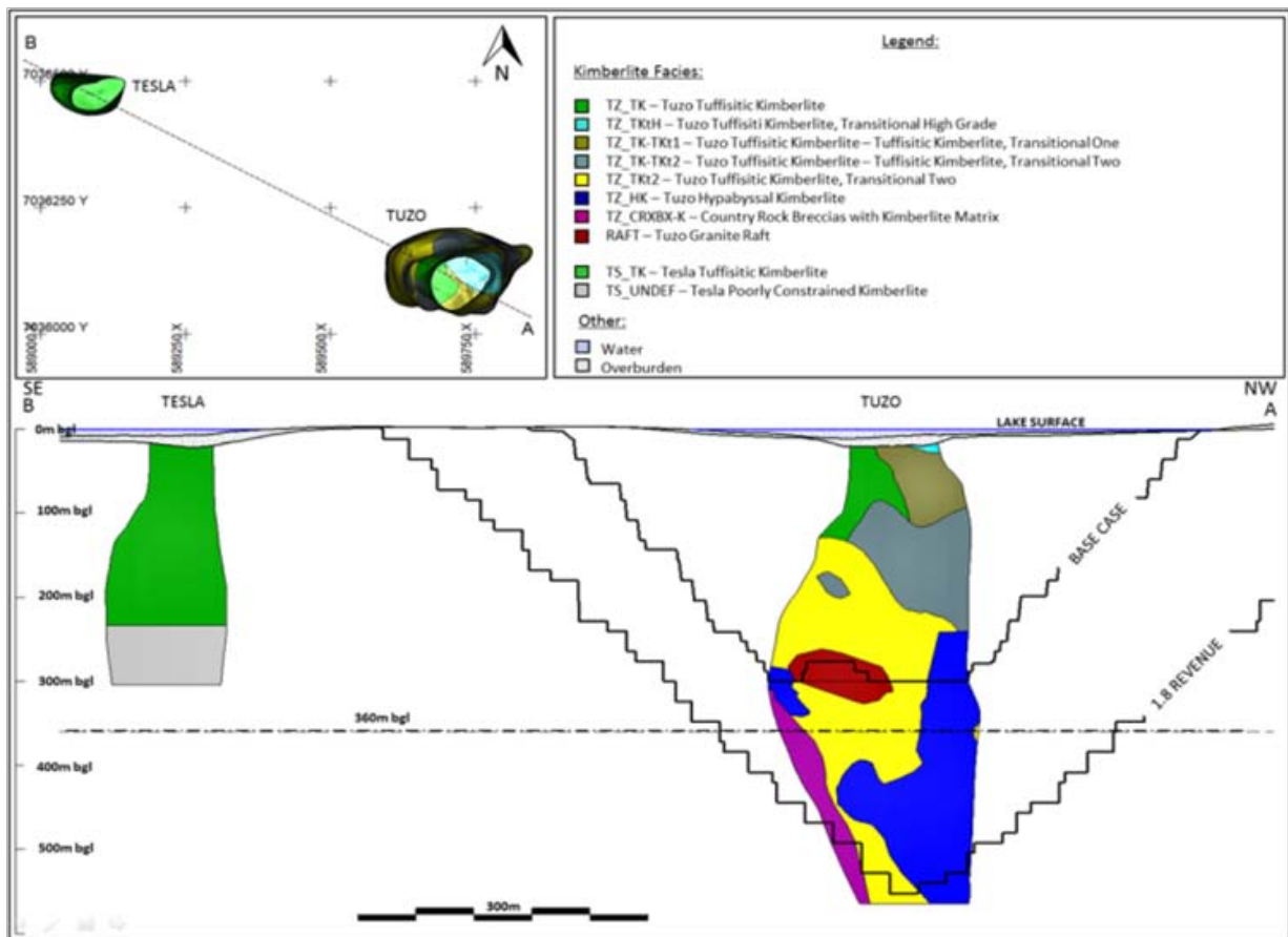
Figure 7-10: Tuzo Kimberlite
