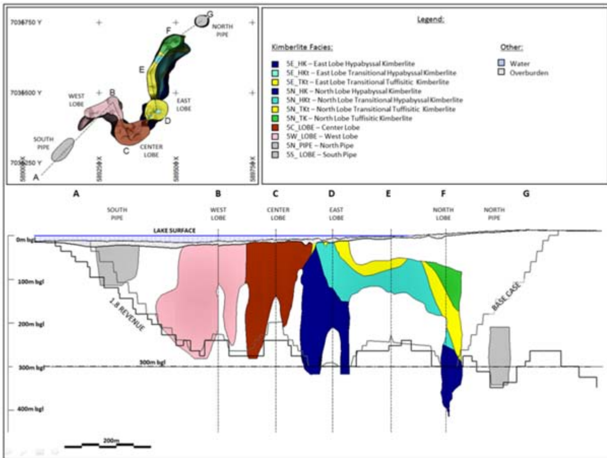
Figure 7-9: 5034 Kimberlite
