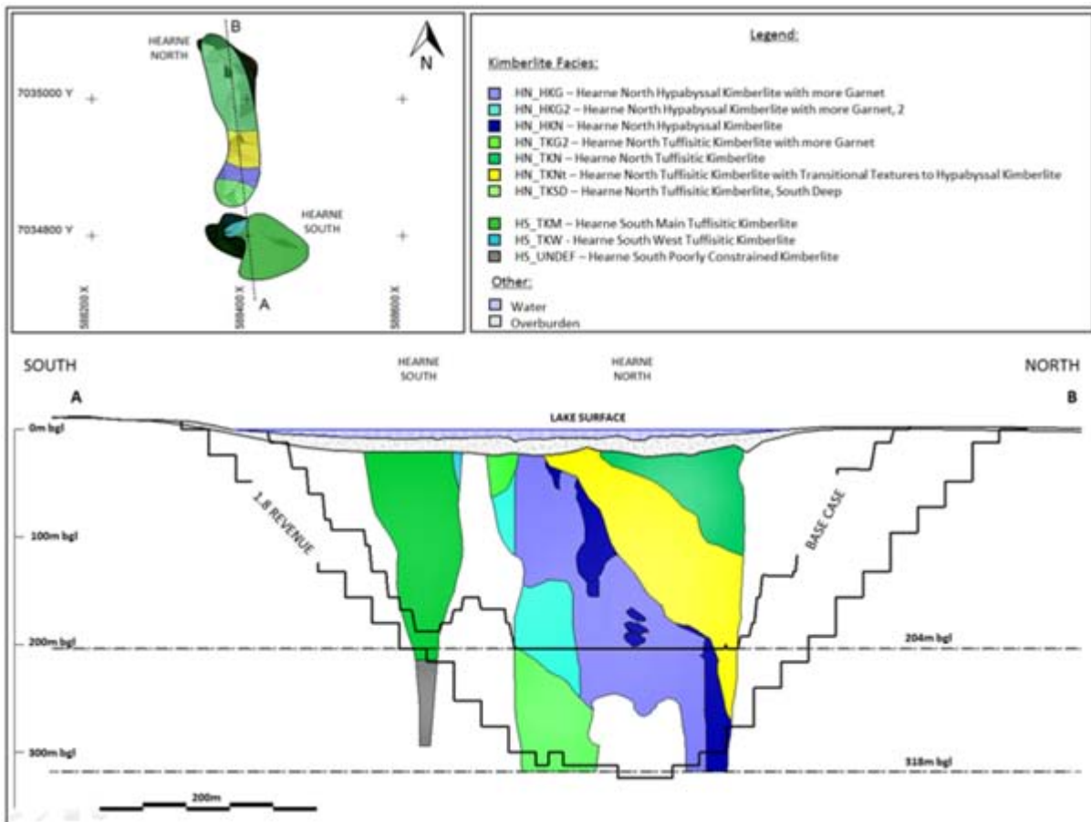
Figure 7-8: Hearne Kimberlite
